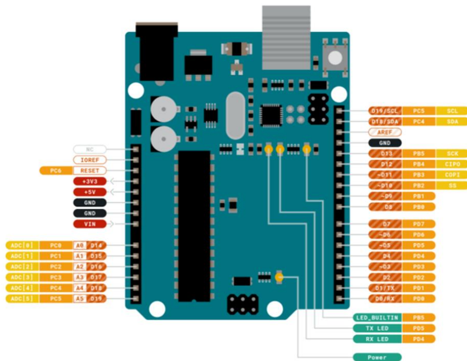
Figure 46: Pinout of the Arduino Uno
