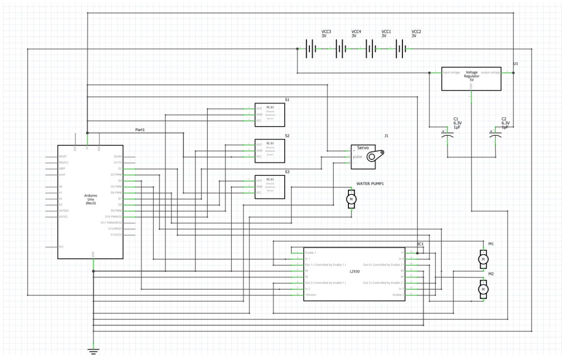
Figure 72: Schematic of Project Design
