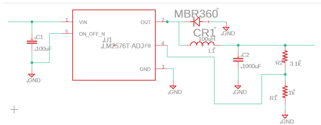
Figure 67: Schematic of the Voltage Regulator Designed Using the Eagle Software
