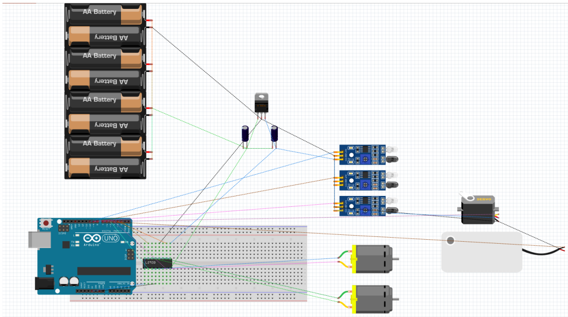
Figure 71: Breadboard Representation of Project Design
