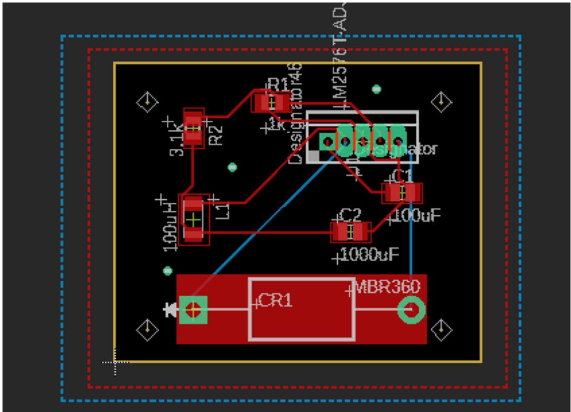
Figure 68: PCB Design of the Switching Voltage Regulator
