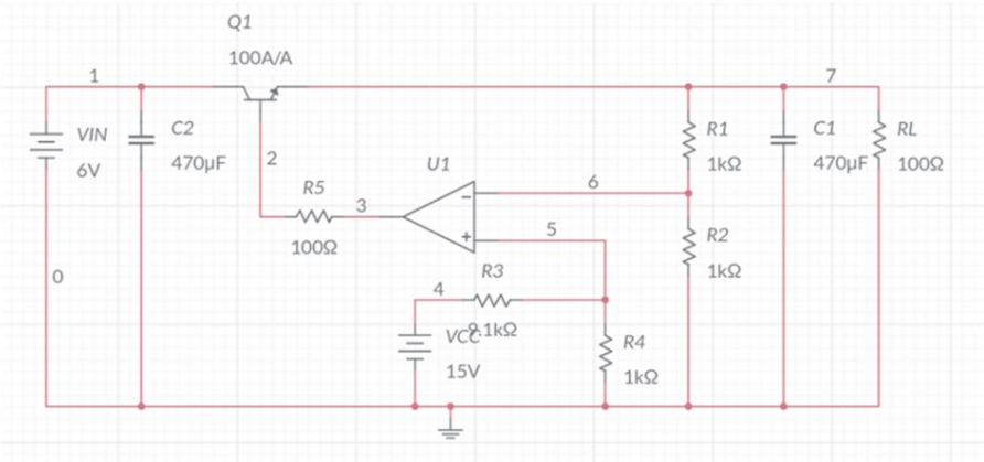
Figure 63: Schematic of the Linear Voltage Regulator.
