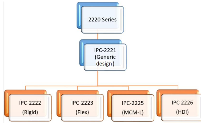
Figure 40: Hierarchy of 2220 Series
