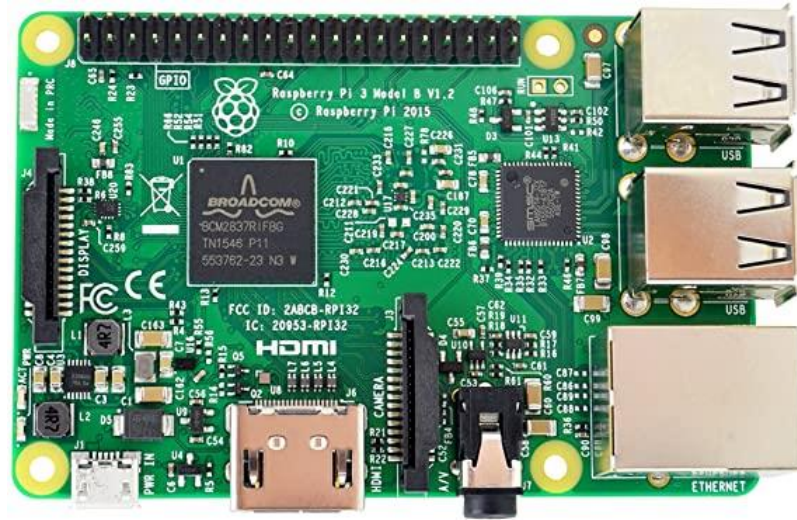
Figure 27: Raspberry Pi 3 Microcontroller
