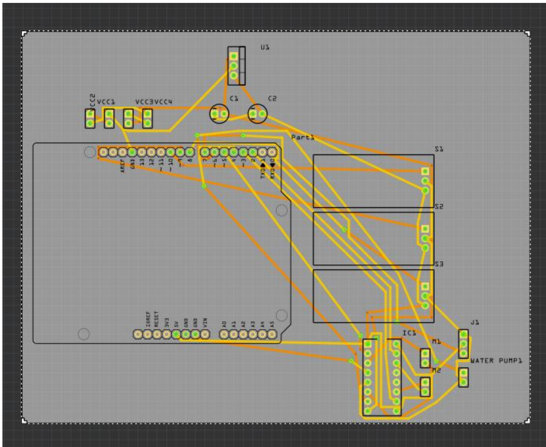
Figure 73: PCB of Fire Extinguishing Robot
