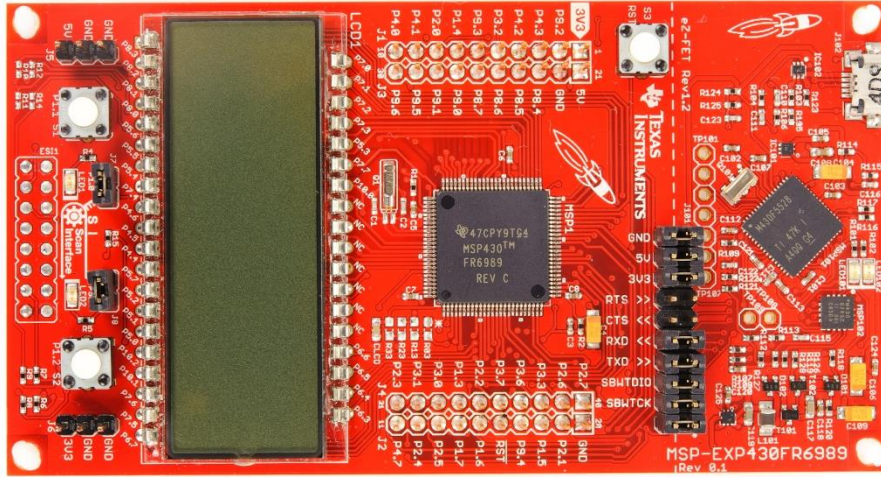
Figure 28: MSP430F6989 Microcontroller
