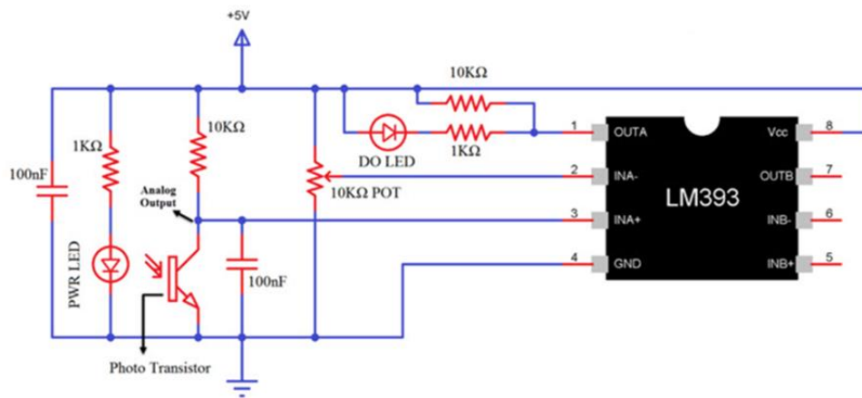
Figure 14: Circuit Diagram of Flame Sensor
