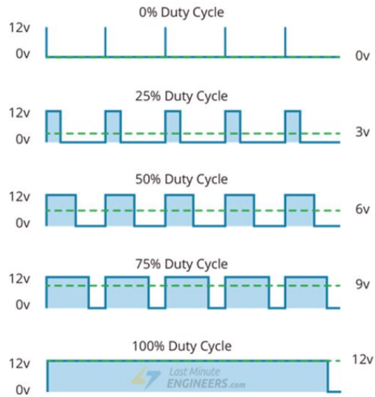
Figure 49: PWM Technique
