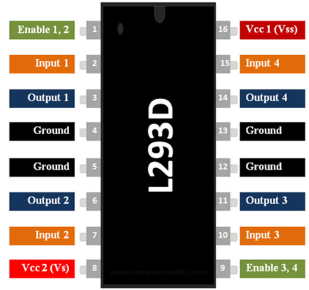
Figure 48: Pin Connections of L293D Motor Driver
